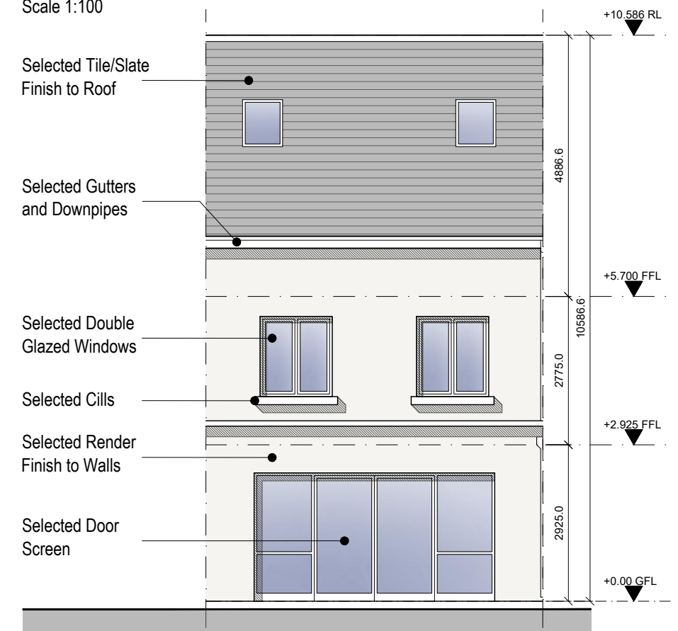
Type A2.2 Rear Elevation
